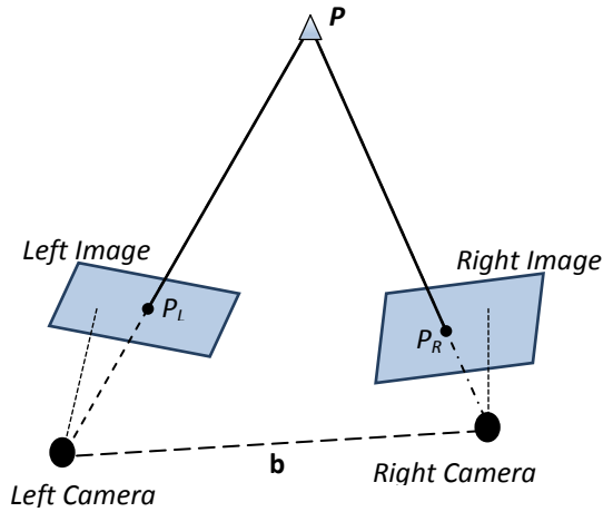
Figure 1. Epipolar geometry
