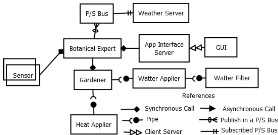
Fig. 4. The architectural view of the system built by the tool
